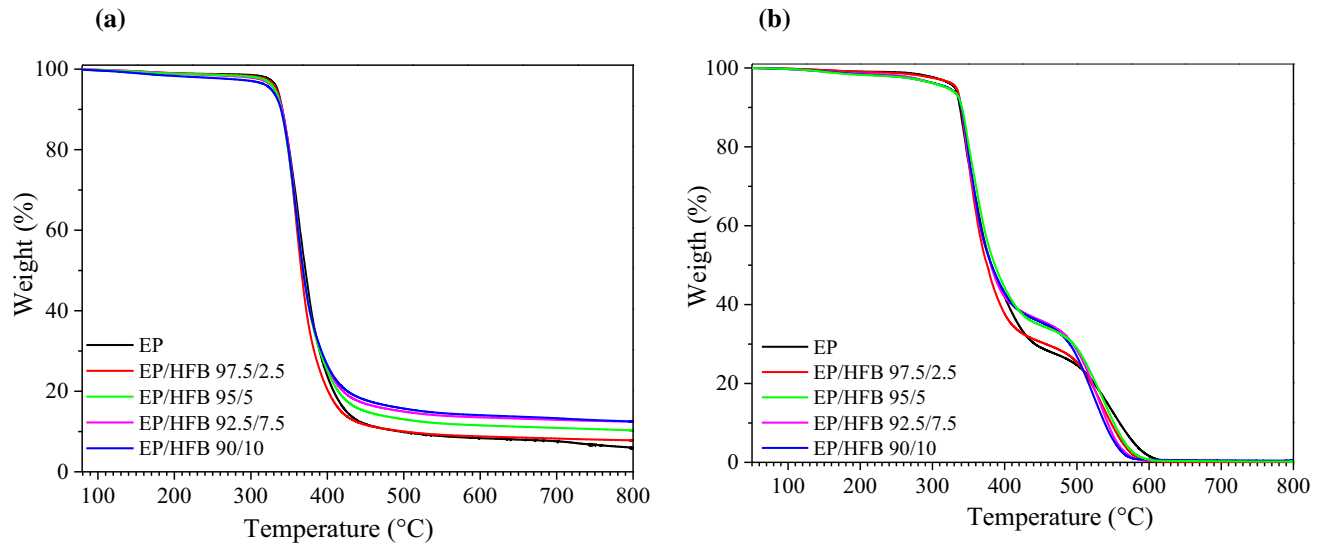
Figure 5 TGA analysis of epoxy/HFB composites run in a nitrogen and b in air.
